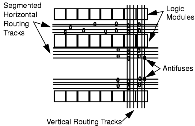
Figure 18 • Routing Structure
