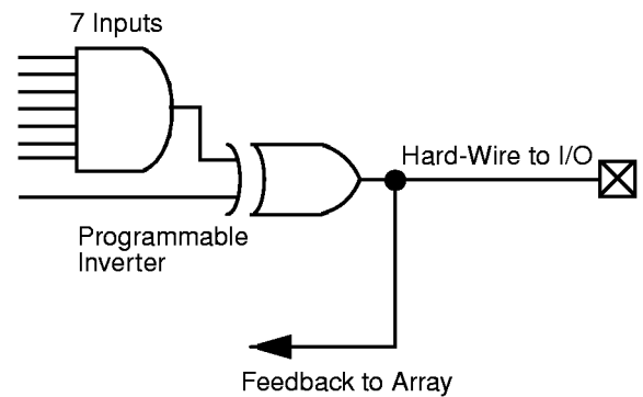
Figure 15 • D-Module Implementation
