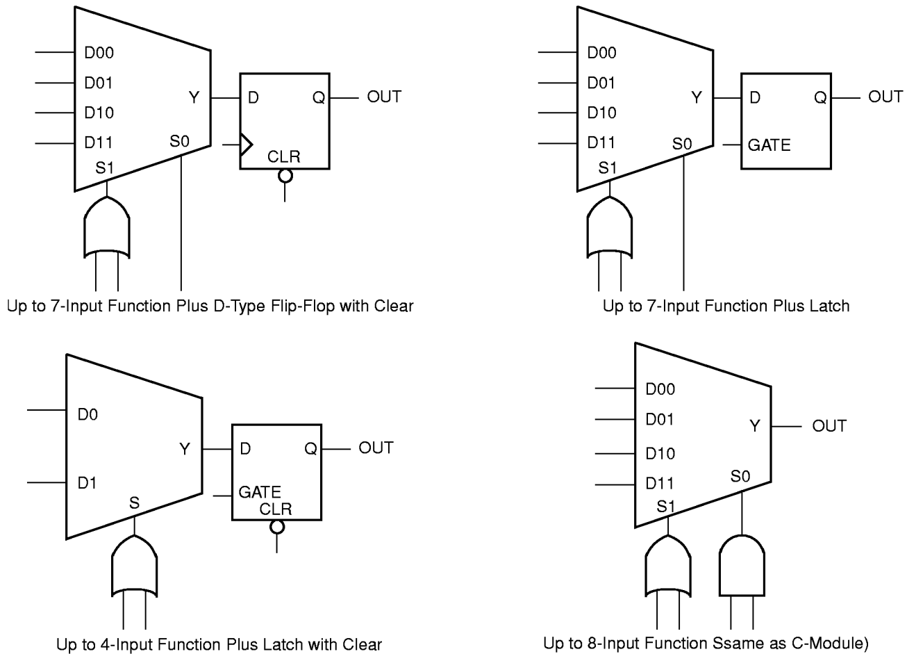
Figure 14 • S-Module Implementation
