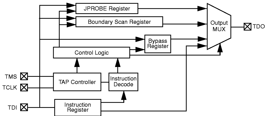
Figure 21 • JTAG BST Circuitry
