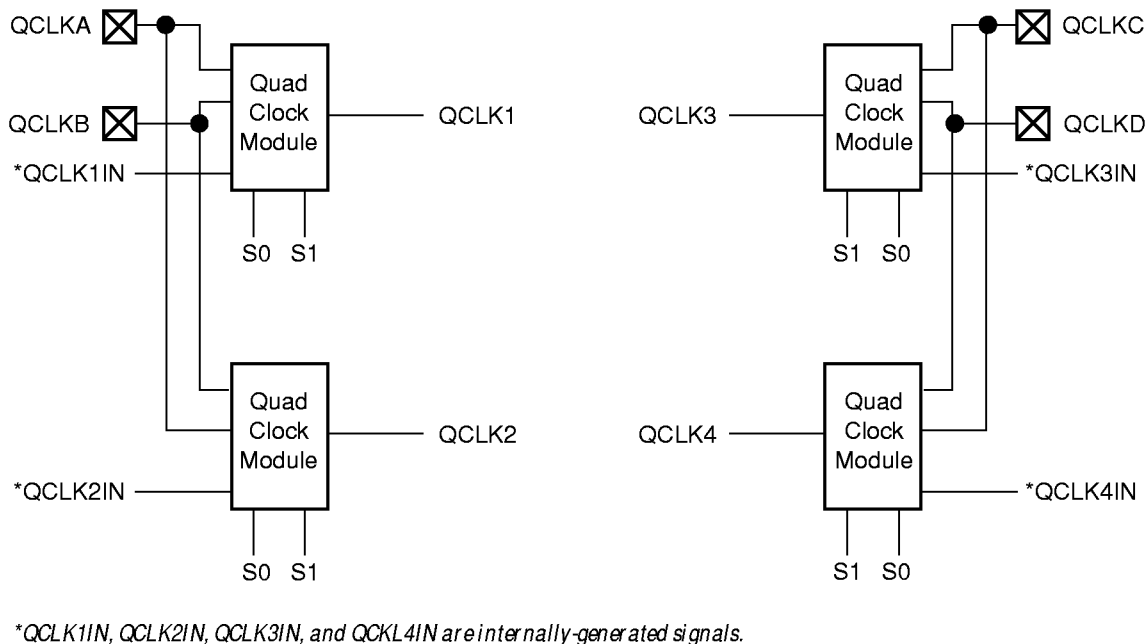
Figure 20 • Quadrant Clock Network
