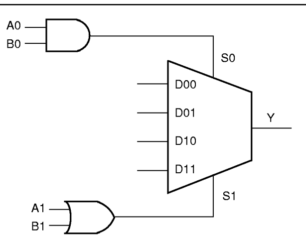
Figure 13 • C-Module Implementation
